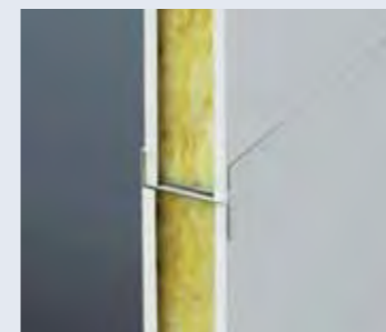
Wall panels joined by H channels. Detail of the glass-wool insulation. Unión de paneles con perfiles en H. Detalle con aislante de fibra de vidrio.
